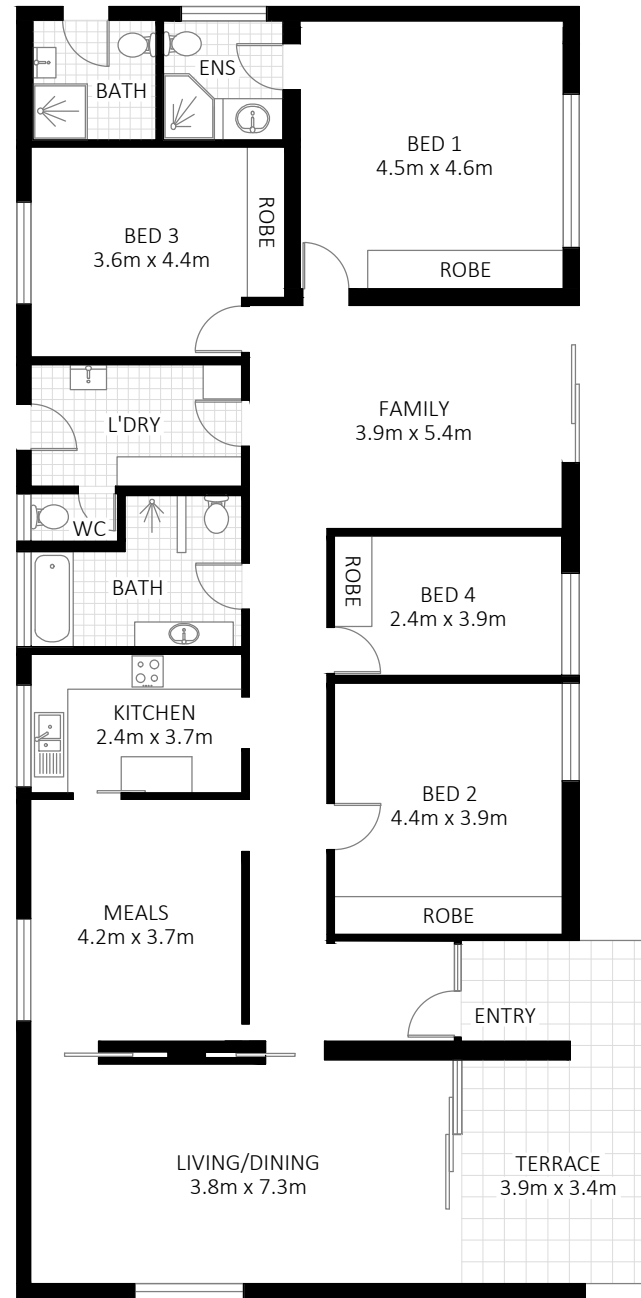
FLOOR PLAN
